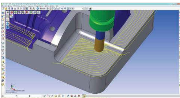
Waveform Machining
