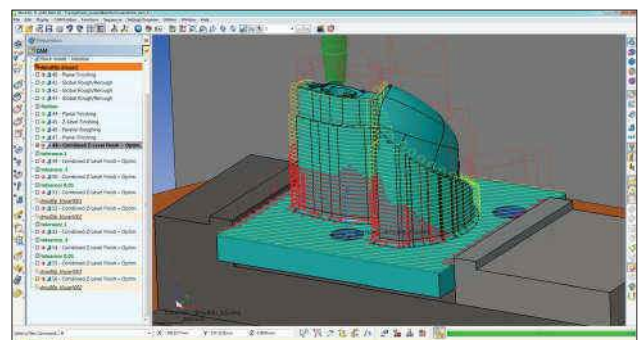
Collision Detection
